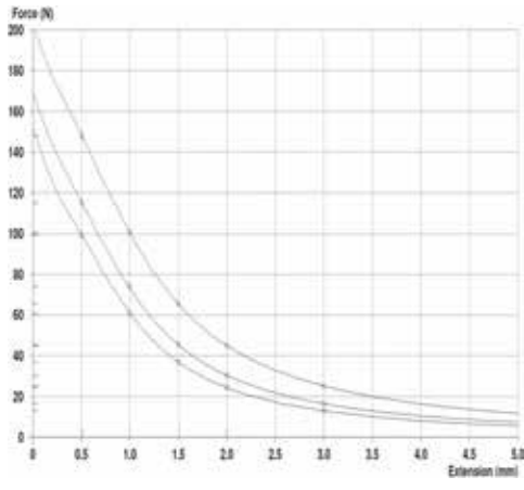
1.8mm Working Stroke, 38 Watt Coil
