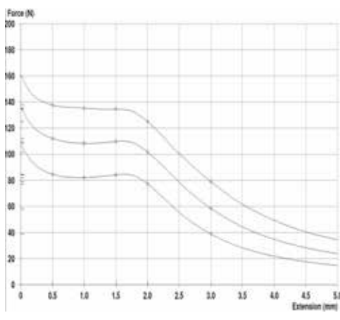
1.8mm Working Stroke, 38 Watt Coil
