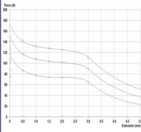
3.0mm Working Stroke, 44 Watt Coil
